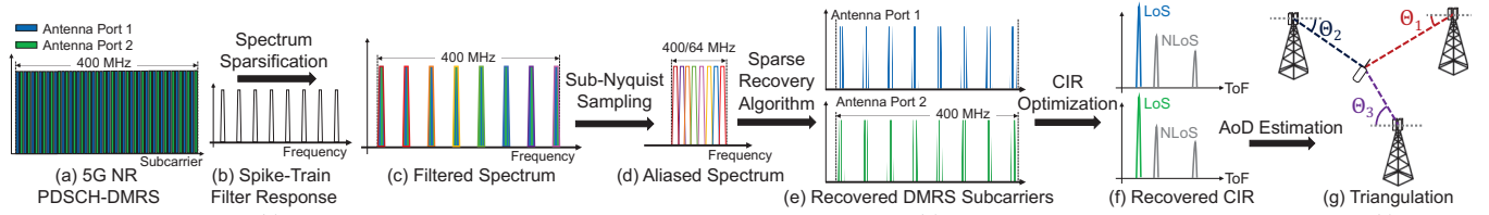
Figure 1: mm-ISLA pipeline. (a) Wideband 5G NR PDSCH-DMRS Spectrum Allocated to 2 Antenna Ports. (b) MEMS Spike-Train Filter Frequency Response. (c) Filtered Sparse Spectrum. (d) Sub-Nyquist Sampled Spectrum Aliased to the Narrow ADC Bandwidth. (e) Recovered DMRS Subcarriers. (f) Recover Channel Impulse Response. (g) AoD-Based Triangulation Localization.
